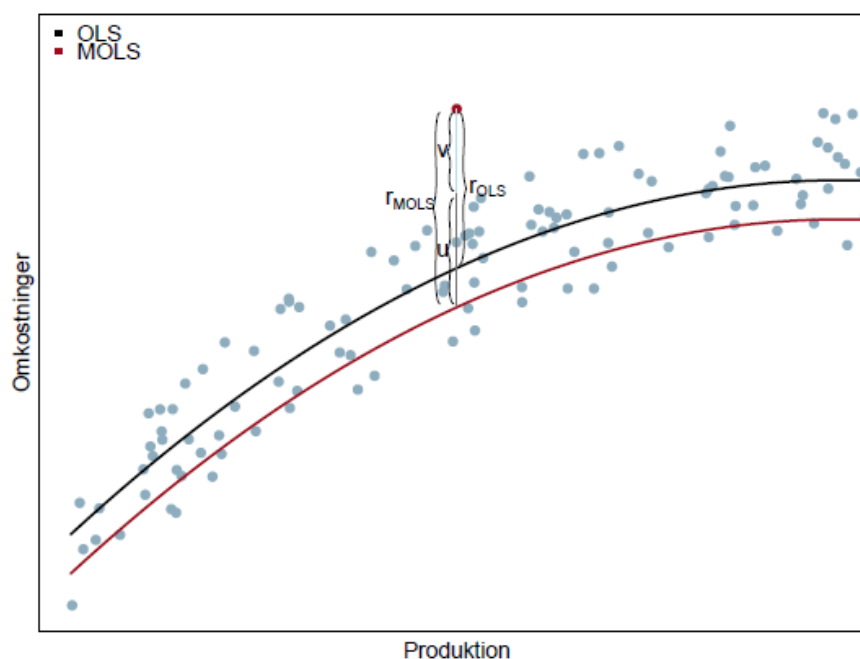
Figur 6.1 MOLS vs OLS
